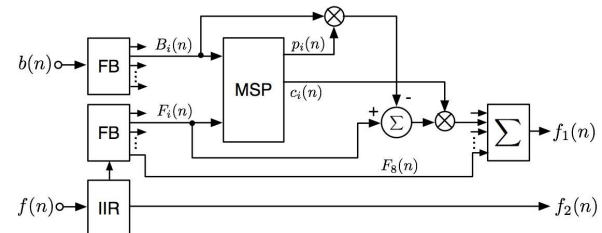
Figure 4: Schematic diagram of the processing that is applied to the forward and backwards facing signals f(n) and b(n) to generate the output signals. FB, IIR, and MSP denote filterbank, IIR filters, and microphone signal processing, respectively
