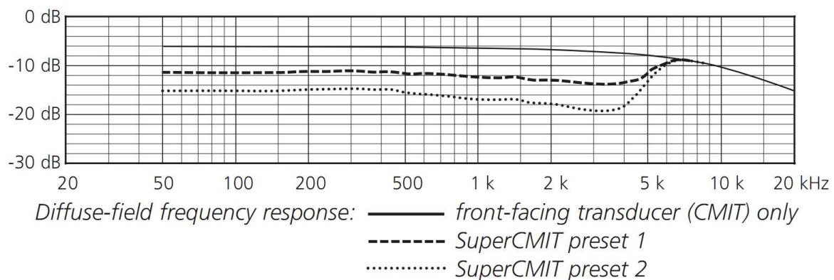
Figure 7: Diffuse-field frequency responses of SuperCMIT ch2, SuperCMIT ch1 Preset 1, SuperCMIT ch1 Preset 2.
