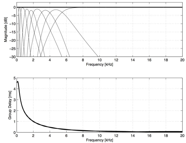
Figure 3: Magnitude response of the subbands (thin, top), filter bank output (bold, top), and group delay (bottom) are shown
