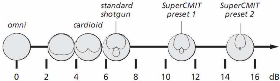
Figure 8: Free-to-diffuse field ratio for first-order directivities and SuperCMIT beamformers
