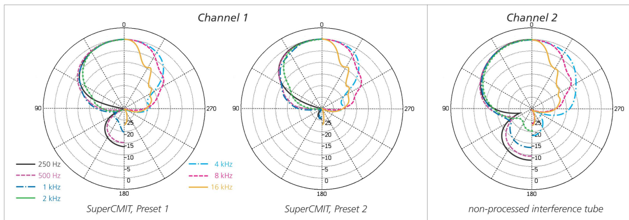
Figure 6: Polar patterns of SuperCMIT beamforming channel (left diagram), enhanced beamformer channel (right diagram).
