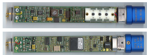
Figure 2: SuperCMIT printed circuit board, top and bottom view
