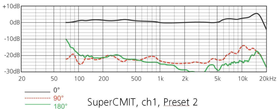
Figure 5: Free-field frequency responses of the SuperCMIT at three sound incidence angles (black—0°, red—90°, green—180°):
