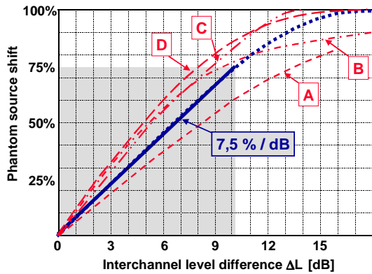
Figure 3-4: from (Wittek and Theile, 2002): Relative phantom source shift A_{\Delta L} = f(\Delta L) . Dotted thick curve after (Wittek and Theile, 2000b) with shift factor Z_{\Delta L} = 7.5 \% /dB. The exact value in Wittek and Theile (2000b) is 7.3%.
