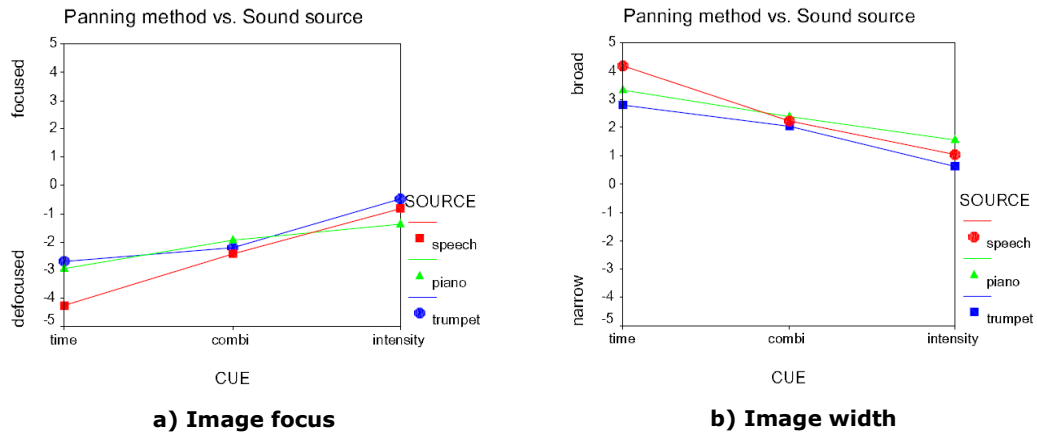
Figure 3-7: from Lee and Rumsey (2004): Subjective comparison of different panning techniques (phantom source at +20^\circ , two-channel loudspeaker setup at \pm 30^\circ ). Attributes: a) image focus, b) image width. The mean of the data is shown.
