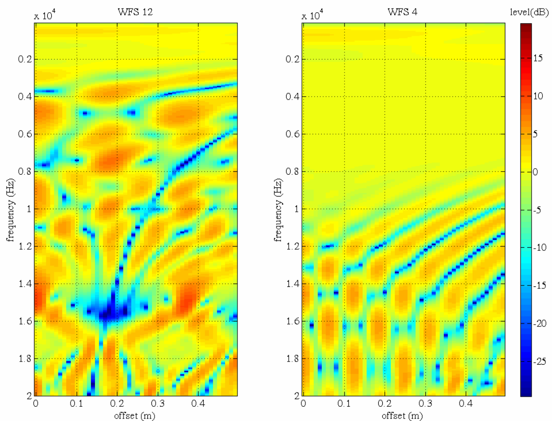
Figure 7-7: Frequency spectra of a WFS virtual source (1 m behind the array) at a line of receiver positions z=2 m. Left diagram: WFS_12; \Delta x=12.67 cm; f_{alias}=2.5 kHz. Right side: WFS_4; \Delta x=4.22 cm; f_{alias}=7.5 kHz.
