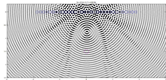
Figure 4-11: Snapshot of the pressure field in the horizontal plane of WFS array of 32 loudspeakers (small circles, \Delta x=12 cm), focussed source 75 cm in front of the array, sine wave of f=4300 Hz ( >f_{alias} except close to the source)
