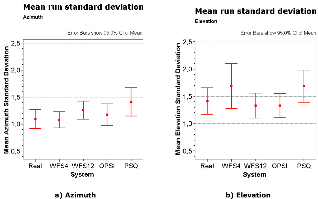
Figure 7-17: Mean run standard deviation \langle \bar{s} \rangle of the perceived azimuth angles, mean of all directions. a) azimuth, b) elevation.
