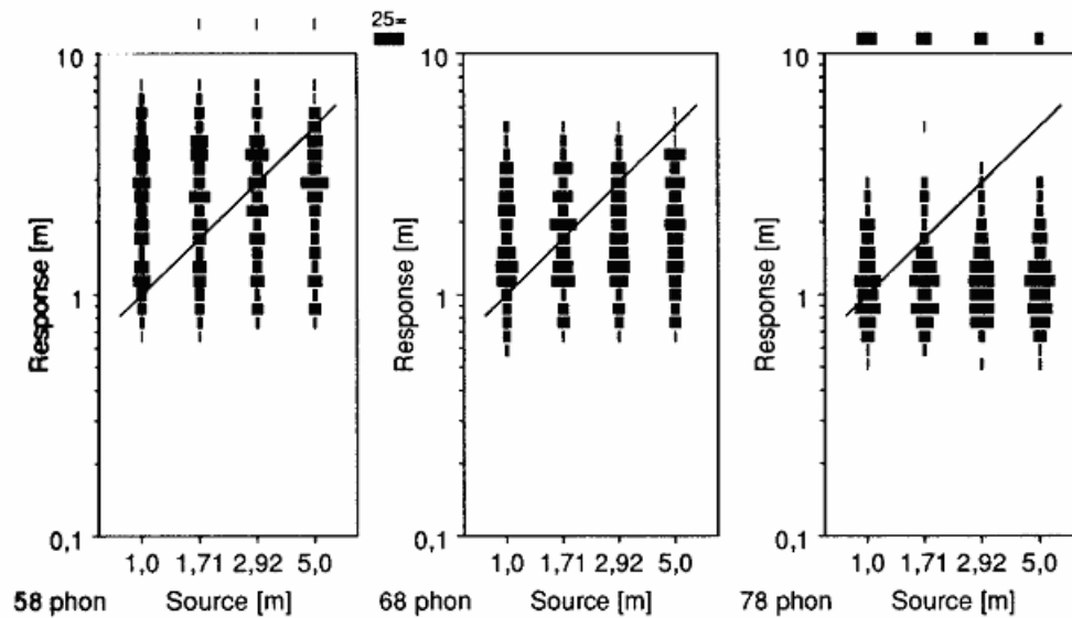
Results for Main 2, anechoic room, voice signal at 45°, all three levels, all subjects.
