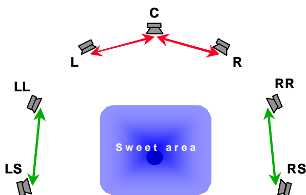
Fig 24: Optional speaker arrangement according to ITU-R 775
