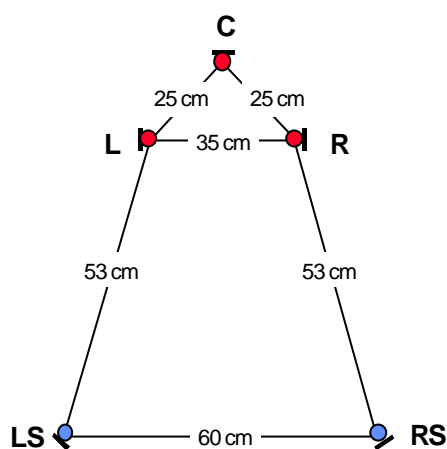
Fig 25: Configuration “INA 5” [14]
