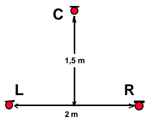
Fig 10: Widely spaced omnis (“Decca-Tree” [11]) Three omni-directional microphones are widely spaced in a triangle configuration. Due to the wide spacing the configuration is not suitable for accurate stereophonic directional imaging. It is used to produce an open, spacious sound, combined with a solid central image. - A similar triangle configuration is applied in the Fukada-Tree [18], however, cardioid microphones are used.
