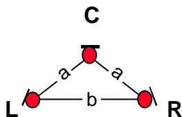
Fig 8: Configuration “INA 3” on the basis of [15] The triangle arrangement has been designed in line with the so-called “Williams -Curves” [15] aiming optimum attachment of the recording areas for L-C and C-R. In [14] the distances a and b are calculated for cardioid capsules dependent on the resulting recording angle \varphi :
