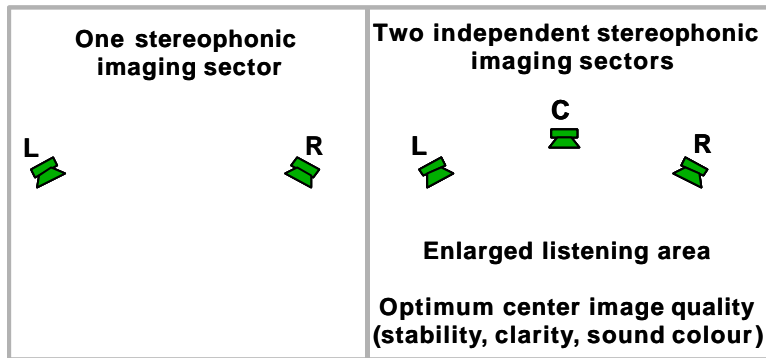
Fig 3: Two vs. three front channels The primary purpose of the center channel C is to divide the stereophonic loudspeaker basis into two stereophonic “sub-areas” [7], using the two 30° imaging sectors L-C and C-R instead of one 60° imaging sector L-R, in order to increase directional stability (to broaden the listening area) as well as to improve “clarity” and “sound colour” of the image in the center area.
