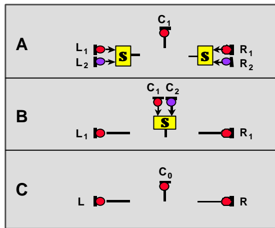
Fig 17: Alternative OCT configurations for improved bass response
