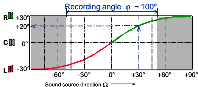
Fig 11: Desirable localisation curve
