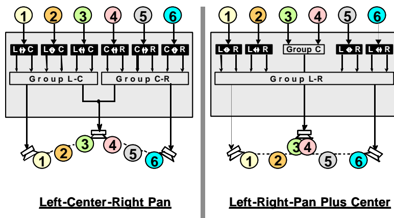
Fig 4: True L-C-R stereophony vs. L-R stereophony plus C Left side: The center channel C offers increased directional stability of the complete L-C-R stereophonic image, which is divided into two stereophonic sub-areas. Right side: The center channel C is used for a stable center image (e.g. soloist), in addition to the usual two-channel stereophonic representation of the orchestra.
