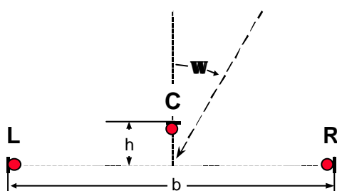
Fig 13: OCT - an optimized triangle configuration
