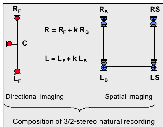
Fig 34: Distinct psychoacoustic functions are applied separately for natural recording
