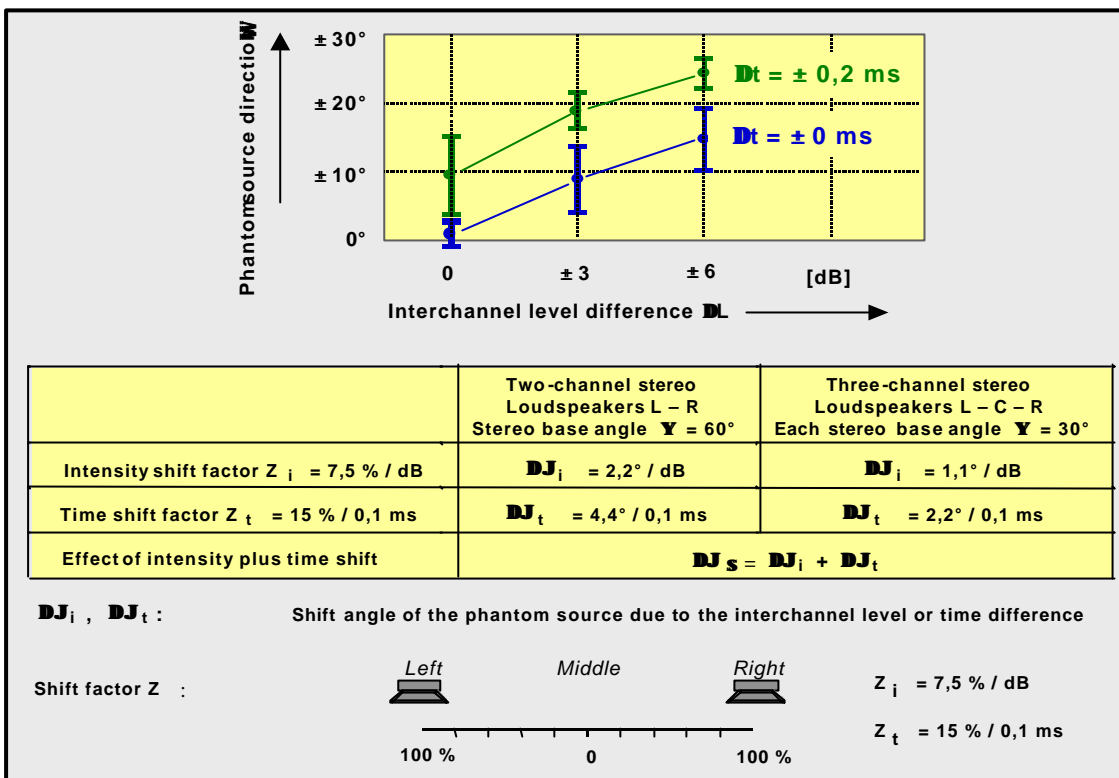
FIG. 14: Intensity and time shift factor
