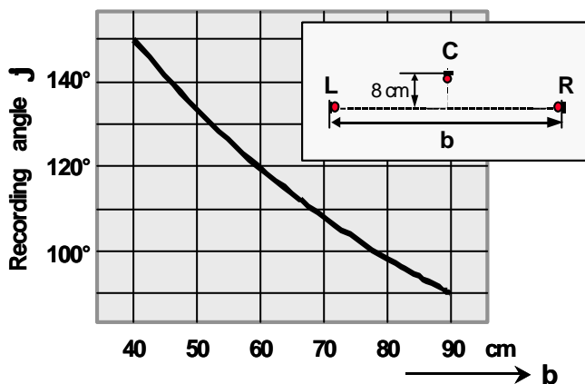
Fig. 15: OCT recording angle as a function of distance b of the capsules L and R. L, R: Super-cardioid C: Cardioid
