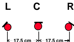
Fig 9: Near-coincident configuration [17] Three microphones in line. The outside capsules L, R have a super-cardioid polar characteristic ( 30^\circ off-center). This avoids producing a strong center phantom image. The center capsule has a cardioid polar characteristic.
