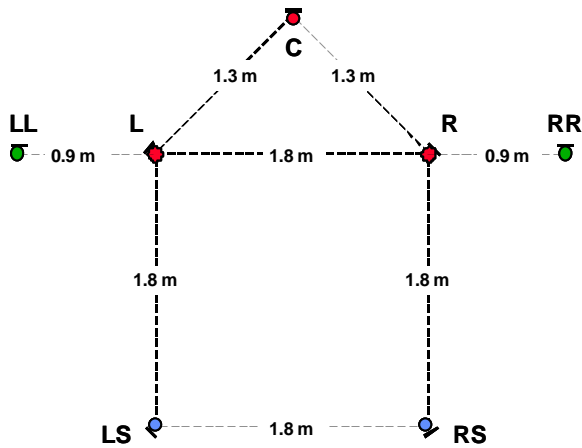
Fig. 26: “Fukada-Tree” [18]
