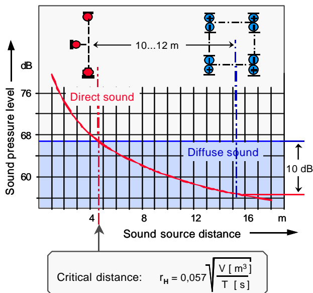
Fig. 33: R/D-ratio and critical distance in the hall 4
